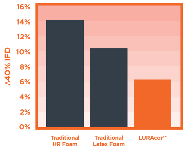
Durability is measured by the % change in 40% IFD after 8,000 cycles of constant force pounding via ASTM 3474-11 Part I3
