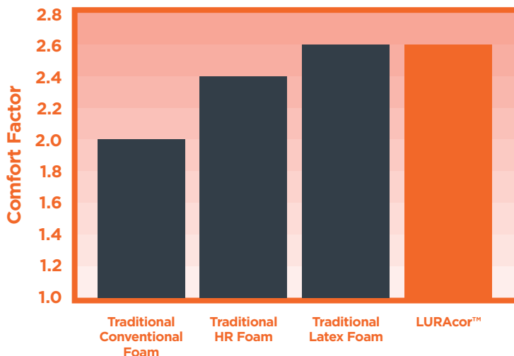
Comfort factor is defined as the ratio of 65% IFD to 25% IFD. IFD is measured via ASTM 3574-11 Test B1
